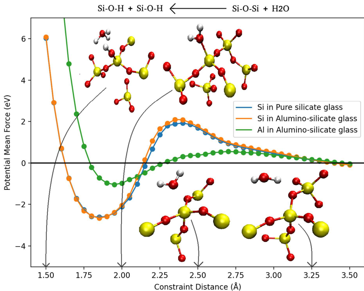
Figure 3. Average activation barrier for dissociating Si in pure silicate, Si and Al in aluminosilicate glass. Blue – bond dissociation around Si in pure silicate glass; orange – bond dissociation around Si in aluminosilicate glass; green – bond dissociation around Al in aluminosilicate glass. The H 2 O molecules approaching towards the Si–O–Si bridge is visualized at each step and the constraint distance of the snapshots are pointed by the arrows.
