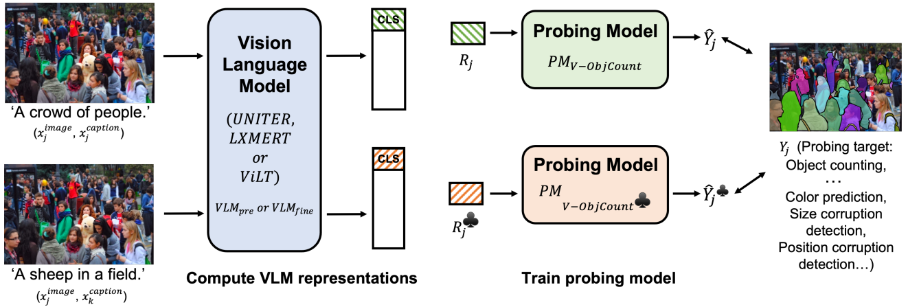
Figure 1: Probing methodology: The first step is to compute the final layer representations of the image/caption input using the chosen Vision Language Model. Then, we use the final layer [CLS] or word token representations R_j to train a linear probing model on the probing task. This example illustrates the methodology using the visual probing task V-ObjCount and an image from MS-COCO. This task consists in counting the number of objects in an image using (x_j^{image}, x_j^{caption}) as input and Y_j as target. The notation \clubsuit indicates the corresponding task (V-ObjCount) with mismatched instances (i.e. a caption that does not match the image and label), which uses (x_j^{image}, x_k^{caption}) as input and serves as a baseline.
