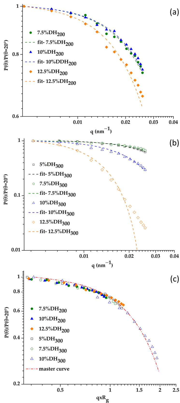
Figure 3. Dependence of experimental normalized form factors ( \frac{P(\theta)_{\text{exp}}}{P(\theta=20^\circ)_{\text{exp}}} ) and the corresponding fit on (a,b) scattering vector ( q ) and (c) qxR_g of dextran-based diblock copolymers nano-objects prepared by photo-PISA.
