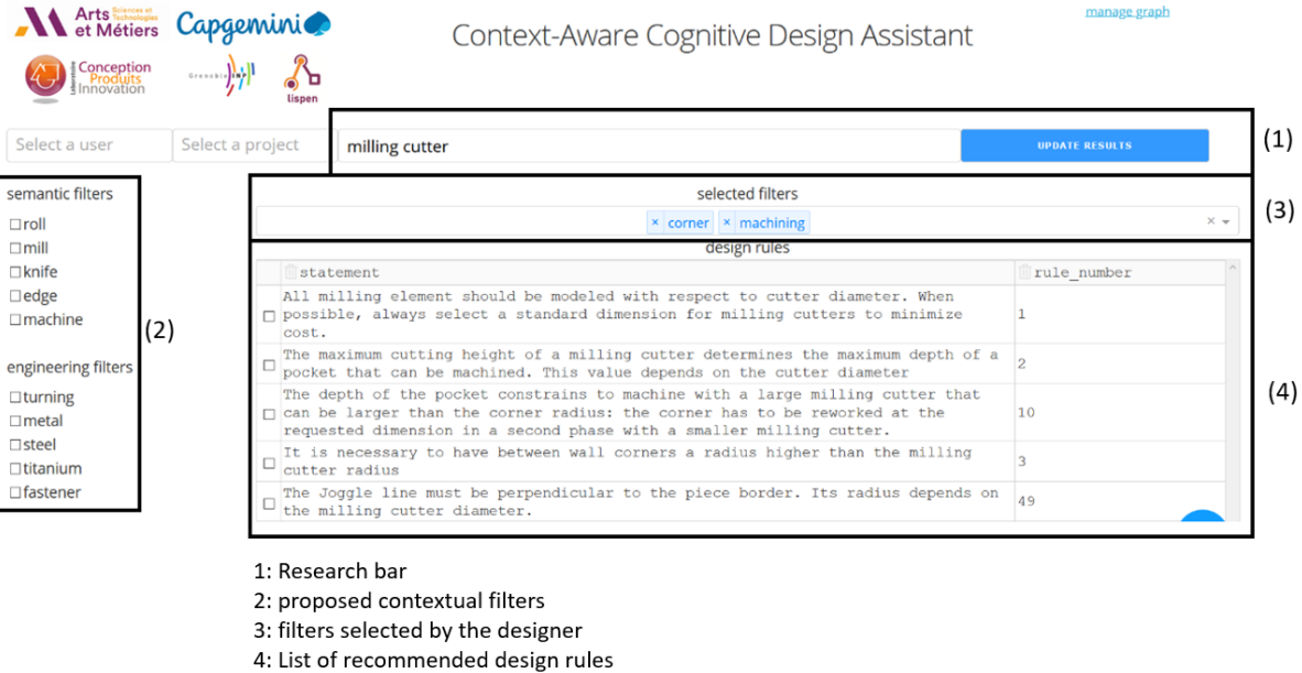
Figure 7 : Dash web interface
