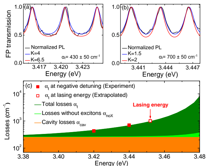
FIG. 4. Modeling of the Fabry-Perot modes of the 20 \mu\text{m} -long cavity at T = 70 K. (a,b) Experimental estimate of the FP transmission (black line), and its fit for various coefficient of finesse K (red and blue lines); (c) Calculated contributions to the total losses \alpha_t (dark green curve), from Elliott-Tanguy model, compared to experimental total losses deduced from FP transmission (red square dots). The open red square dot corresponds to the extrapolated total losses at the lasing energy \alpha_t = 1000 \pm 100 \text{ cm}^{-1} .
