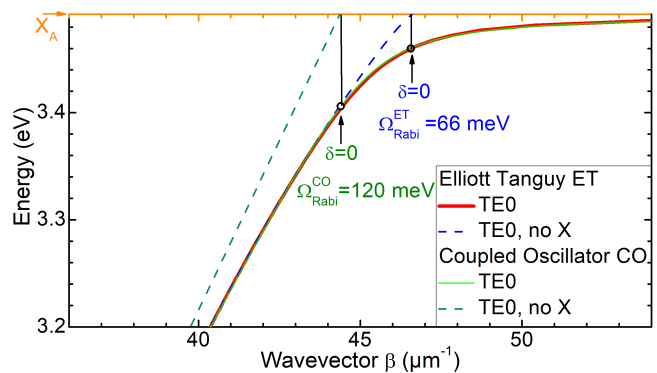
FIG. 9. Comparison of the coupled oscillator model and the Elliott-Tanguy model of the TE0 modes of the polaritons dispersion. The corresponding bare waveguide modes are indicated as dashed lines, and the A exciton energy as a horizontal orange line. The vertical black lines indicate the zero-detuning condition for each model, and the associated Rabi splitting.
