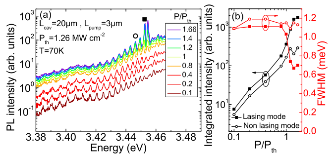
FIG. 2. Laser operation of the 20 \mu\text{m} -long cavity at 70K. (a) Power-dependent PL spectra across the lasing threshold; (b) intensity (black) and linewidth (red) of the lasing and the non-lasing modes.
