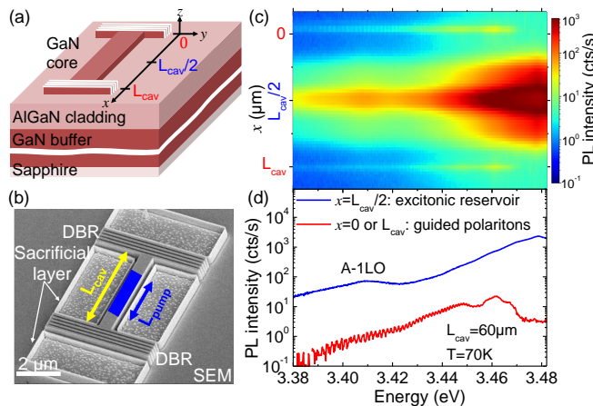
FIG. 1. Sample description. (a) Sample structure: ridge cavity after lithography and deep etching, the guided mode propagates along the x -axis in the GaN core; (b) Scanning electron micrograph image of a 5 \mu\text{m} -long polariton ridge waveguide. The adjustable pump spot is sketched in blue; (c) \mu\text{PL} image of a 60 \mu\text{m} -long cavity excited below lasing threshold, with a line-shaped excitation spot ( L_{\text{pump}} = 6.5 \mu\text{m} ); (d) Emission spectra extracted from (c) at positions x = L_{\text{cav}}/2 (excitation spot) and x = 0 or L_{\text{cav}} (DBR).
