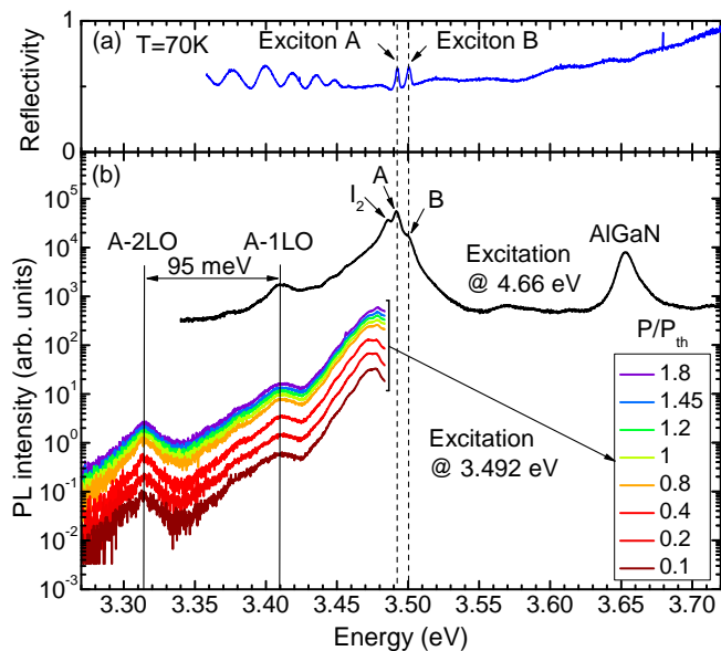
FIG. 8. Low temperature measurements. (a) Reflectivity performed on the same sample. (b) Emission spectra at T = 70 K under non-resonant excitation at 4.66 eV ( i.e. 266 nm laser, black line) and under quasi-resonant excitation at 3.492 eV vs. pump power ( i.e. 355 nm laser, colored lines). The emission is measured at the position of the excitonic reservoir ( x = 0 \mu\text{m} ) of a 20 \mu\text{m} -long cavity.
