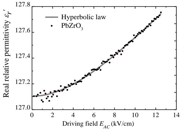
Fig. 4. The real part of relative as the function of the applied AC electric field (black circles). The solid gray line is a fit to the hyperbolic law (1) at 1 kHz.
