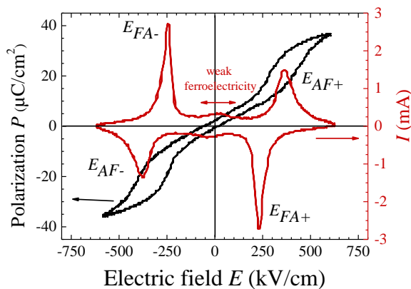
Fig. 2. P - E and I - E loops of the PbZrO 3 sample at 1 kHz. The I - E loop shows a slight increase at zero field corresponding to a weak ferroelectricity
