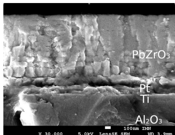
Fig. 1. Cross-section SEM image of the \text{PbZrO}_3/\text{Pt}/\text{Ti}/\text{Al}_2\text{O}_3 sample
