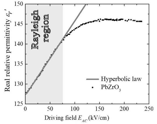
Fig. 5. The Real part of the relative permittivity as the function of the driving field E_{AC} . The solid gray line correspond to the hyperbolic fit.
