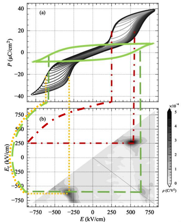
Fig. 3. P(E) loops and FORC distribution of the PZO antiferroelectric thin films. The different lines show the switching fields and the green loop is hypothetic.
