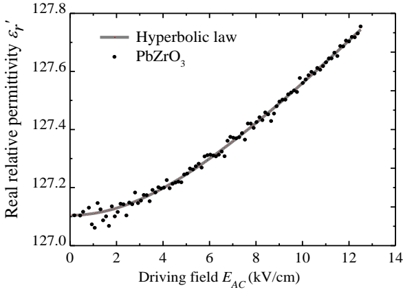
Fig. 4. The real part of relative as the function of the applied AC electric field (black circles). The solid gray line is a fit to the hyperbolic law (1) at 1 kHz.
