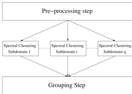
Fig.1 Principle of parallel spectral clustering.
