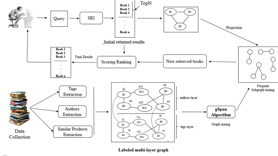
Fig. 1. Architecture of book retrieval approach based on frequent sub-graph mining
