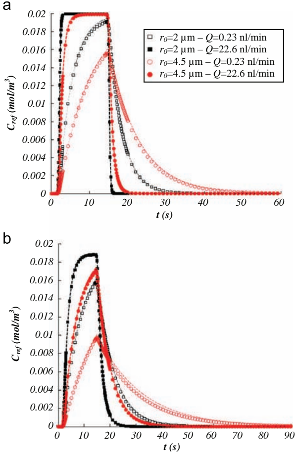
Fig. 5. Numerical simulations: tracer kinetics. Mean concentration of H_2^{15}O in the whole computational domain as a function of time. Results are shown for four combinations of two flow rates (0.23 nl/min and 22.62 nl/min) and two radii (2 \mu m and 4.5 \mu m ). (a) D_e = D_t , \lambda_d = 1 . (b) D_e = D_s/100 , \lambda_d = 0.95 . Symbols: results obtained by numerical simulations. Dashed lines: best fits of the numerical results by Eq. (2) (Pearson's r correlation coefficient is typically greater than 0.98). See inserted legends for details.
