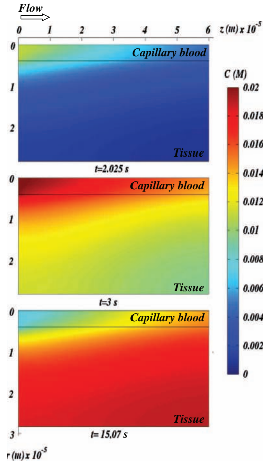
Fig. 3. Numerical simulations: transient concentration fields in the classical Krogh cylinder geometry. \text{H}_2^{15}\text{O} concentration field calculated by numerical simulations in a 4\text{ }\mu\text{m} radius capillary tube with blood flowing at 11.31\text{ nl/min} ( \lambda_d=1 ). Tracer spatial repartition at the very beginning of injection ( t=t_0+0.025\text{ s} , top panel), after one second of infusion ( t=t_0+1\text{ s} , middle panel) and at the very beginning of clearance ( t=t_1+0.07\text{ s} , bottom panel).
