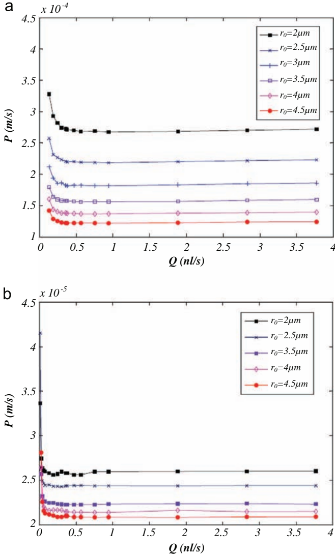
Fig. 8. Renkin-Crone's analysis: permeability coefficient P identified as a function of flow rate for various capillary radii. (a) D_e=D_t , \lambda_d=1 . (b) D_e=D_s/100 , \lambda_d=0.95 . Note that when k_1v/Q > 1 (i.e. at the lowest flow rates), P remains undetermined.
