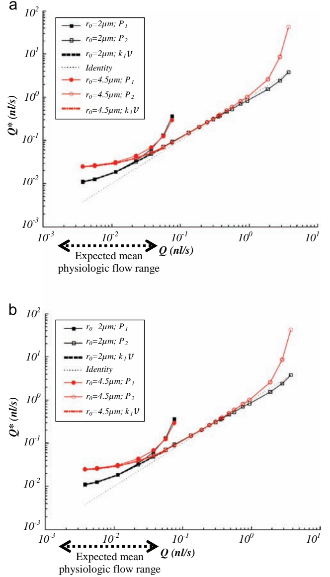
Fig. 9. Renkin-Crone's analysis: flow rate estimated from Eq. (20) as a function of the imposed flow rate for various capillary radii. (a) D_e=D_t , \lambda_d=1 , P_1=1.218 \times 10^{-4} m/s, P_2=2.676 \times 10^{-4} m/s; (b) D_e=D_s/100 , \lambda_d=0.95 , P_1=2.085 \times 10^{-5} m/s, P_2=2.561 \times 10^{-5} m/s. Note that when PS < k_1v , i.e. at high flow rates, Q^* remains undetermined. See inserted legend for details ( k_1v corresponds to the low flow rate, flow-limited asymptotic regime). Bold dotted segment: same convention as in Fig. 7.
