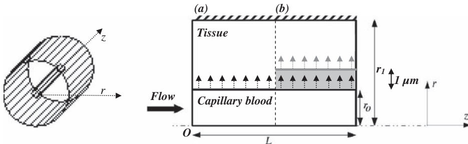
Fig. 2. Krogh cylinder geometry (not to scale) and notations used for the numerical simulations. Left: three-dimensional representation, highlighting a unique capillary surrounded by an isolated tissue cylinder; Right: two-dimensional representation of half the computational domain in the Orz plane. The whole computational domain is constructed by symmetry of revolution around the Oz axis. The total flux at the capillary/tissue interface is given by SJ , where S is the area of this interface ( 2\pi r_0 L ) and J is the surface flux, represented by individual arrows. (a) Classical Krogh cylinder geometry. (b) Variant including a third phase representing the endothelial layer (schematized in gray).
