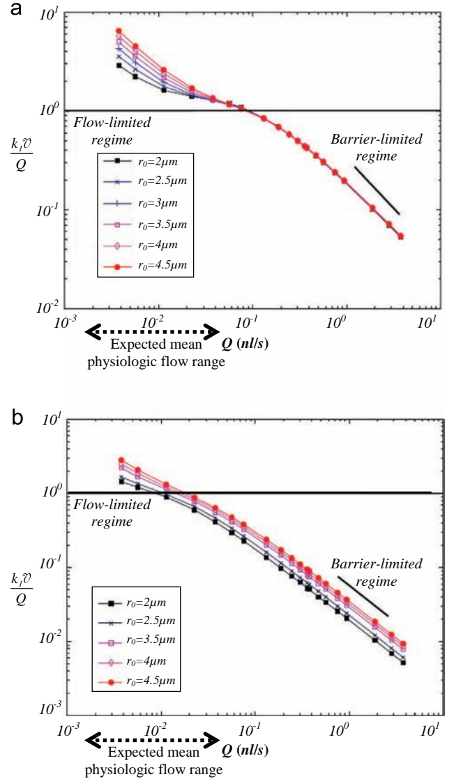
Fig. 7. Renkin–Crone's analysis: parameter k_1 v/Q identified as a function of flow rate for various capillary radii. (a) D_e = D_t , \lambda_d = 1 . (b) D_e = D_s/100 , \lambda_d = 0.95 . The thin line ( k_1 v/Q = 1 ) corresponds to flow-limited regime. The bold line indicates a slope -1 (barrier-limited asymptotic regime). The bold dotted segment indicates the range of mean physiologic flows in capillary vessels (i.e. flow rate range spanned by blue and red lines in Fig. 6).
