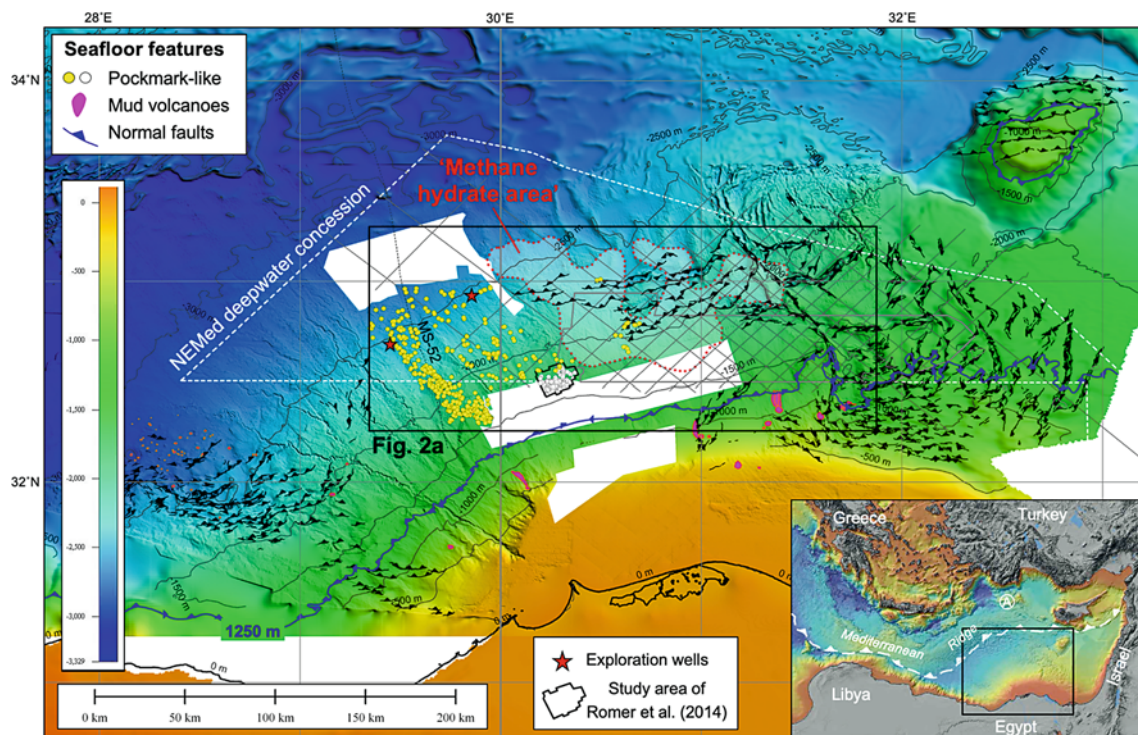
Fig. 37.1 Location of the Nile deep-sea fan showing seafloor bathymetry based on a regional multibeam mosaic (acquired by G eoazur from 1998 to 2011) used to map the indicated seafloor features. ‘Pockmark-like’ features refer to reflective carbonate patches 75–400 m wide of mainly positive relief (yellow dots identified for this study, white dots from the study of R mer et al. 2014). The 1250 m bathymetric contour (highlighted in blue) corresponds to the approximate upper limit of the methane hydrate stability zone. The possible extent of a BSR within the NEMed deepwater concession is indicated
