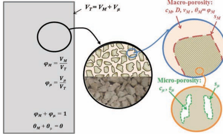
Fig. 2 Schematic representation of the two pore domains in the column. V_T , V_M , and V_\mu are the total, macroscopic, and microscopic volumes, respectively ( L^3 ); \phi_M and \phi_\mu are the volume fraction of macroscopic and microscopic domains, respectively (—); \theta_M and \theta_\mu are the total porosity of the macro and micro-domains, respectively; \varepsilon_M and \varepsilon_\mu are the local porosity of the macro and micro-domain, respectively (—), and \varepsilon_M = 1 , thus \phi_M = \theta_M and \theta_\mu = \phi_\mu \varepsilon_\mu ; c_M and c_\mu are the local concentrations of TCE ( M L^{-3} ) in the macro and micro-regions; s_M and s_\mu are the sorbed concentrations of TCE ( M L^{-3} ) on the cement paste material in the macro-pores and micro-pores region, respectively. On the bottom of the middle drawing is a photograph of the cement paste pieces.
