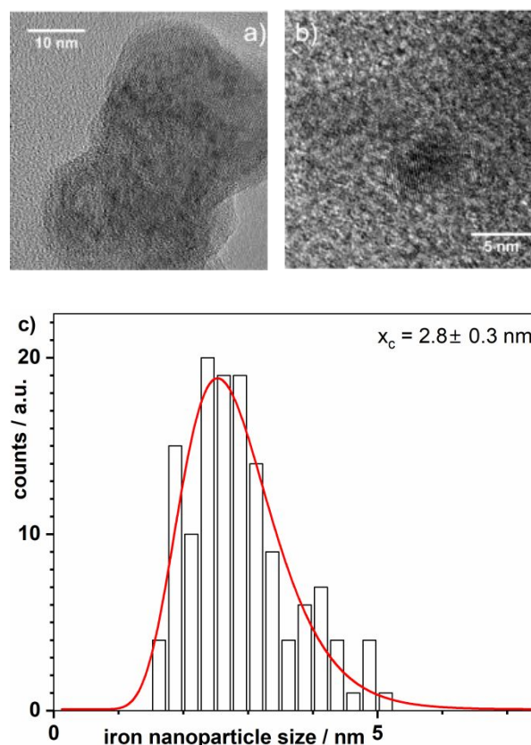
Figure 2. a) HR-TEM images of the composite material Fe(nP)/nC; b) close-up on one Fe(nP) nanoparticle; c) histogram of the size distribution of iron nanoparticles, shown to be centered at 2.8 \pm 0.3 nm based on a log-normal fitting of the data of (non-dimensional) width parameter \sigma=0.1
