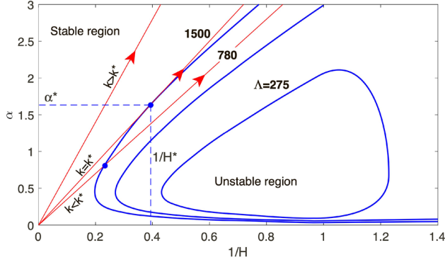
Fig. 3 Marginal stability curves for \beta = 2.25 and \gamma = 0 in coordinates \alpha-1/H . The wavenumber \alpha and 1/H are changing along the straight line as it is shown by the red arrows; \lambda during this evolution successively transfers between stable, unstable and again stable regions
