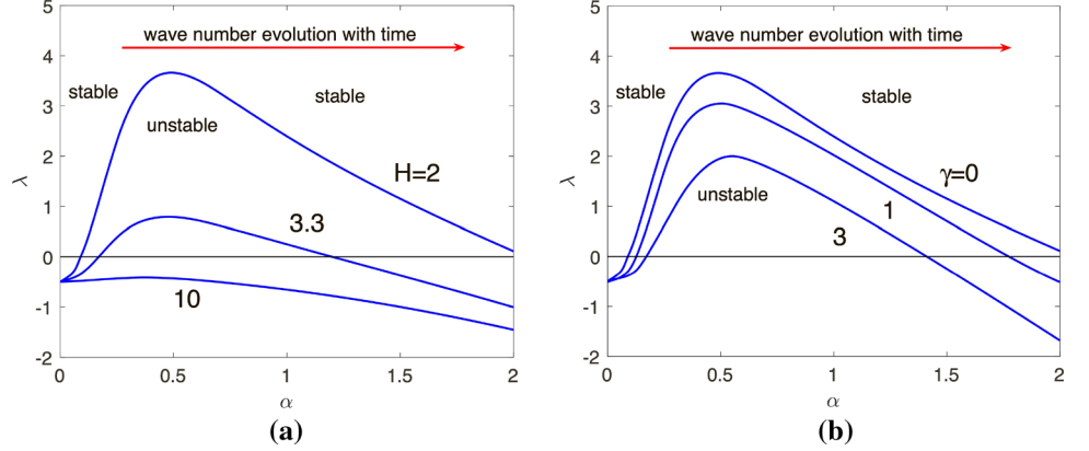
Fig. 2 Growth rate \lambda vs the wavenumber \alpha for \mathbf{a} \Lambda = 1500 , \beta = 2.25 and \gamma = 0 and different values of the dimensionless half-width of the channel H and, \mathbf{b} \Lambda = 1500 , H = 2 and different values of dimensionless viscosity \gamma
