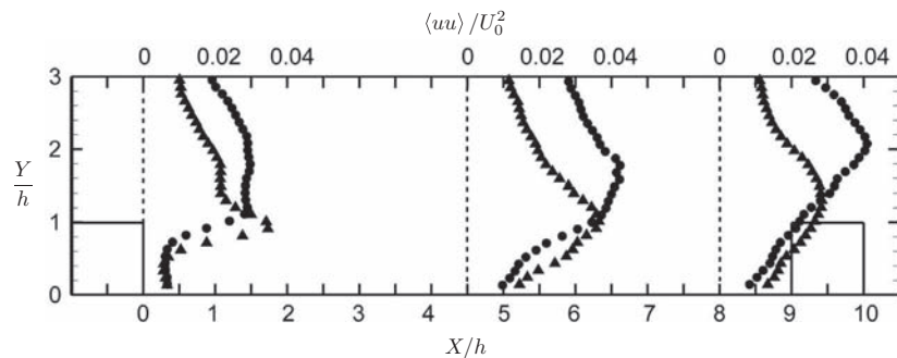
FIG. 8. Profiles of streamwise Reynolds stresses extracted at X/h = 0, 4.5, and 8, for the non-heated leading wall (triangles) and heated leading wall (circles).
