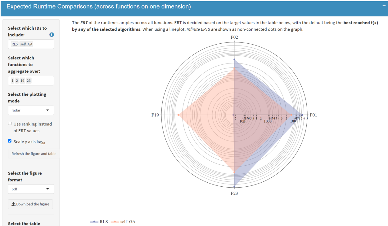
Figure 10: Screenshot of ERT of RLS and the (1, \lambda) GA on four PBO problems, where the ERT values are shown for each selected problem in a radar plot with inverted axis (values are decreasing when moving away from the center). Loosely speaking, an algorithm with a larger span on the plot is considered better, e.g., RLS dominates (1, \lambda) GA on problem F01, F02, and F23 while the latter is superior on F19.
