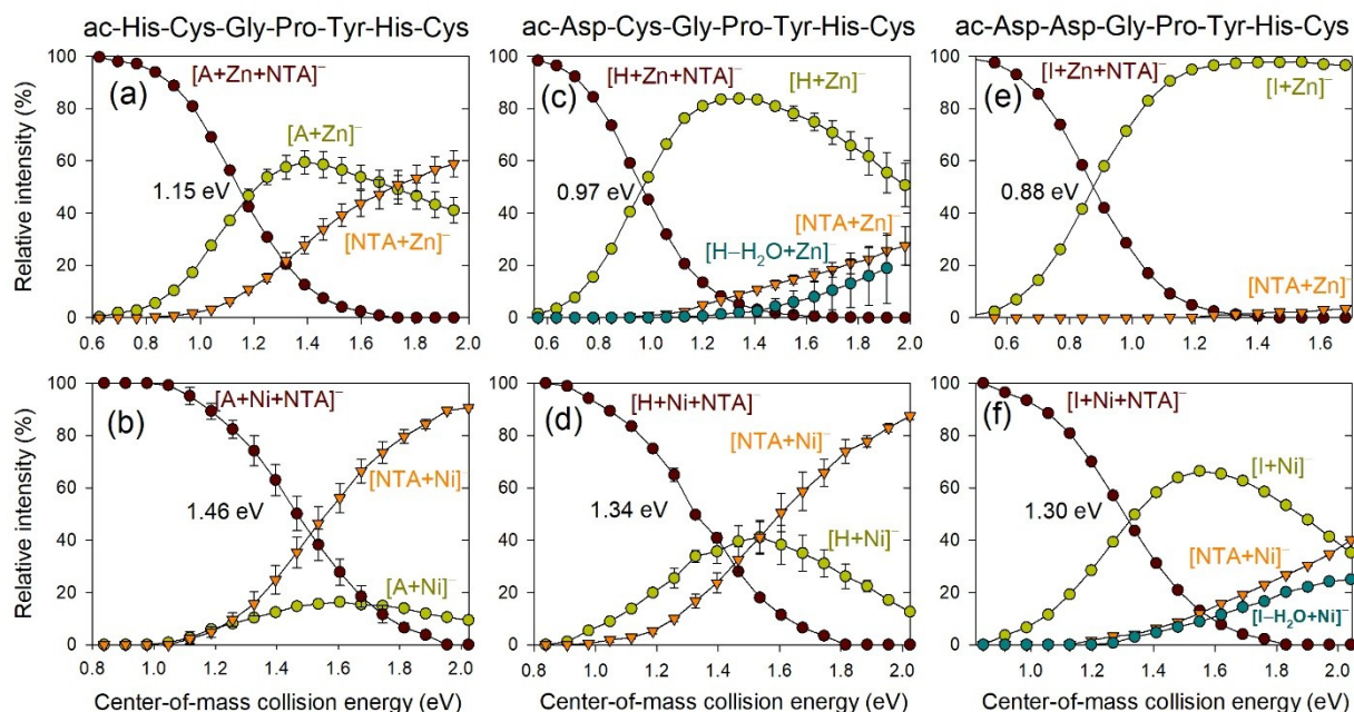
Figure 3. The energy-resolved (c.m./ eV) collision-induced dissociation of [\text{amb}_5\text{-H}+M(\text{II})+\text{NTA-2H}]^- for A , H , and I , where M = \text{Zn} or \text{Ni} , showing the products of [\text{amb}_5\text{-3H}+M(\text{II})]^- , [\text{NTA-3H}+M(\text{II})]^- and [\text{amb}_5\text{-3H-H}_2\text{O}+M(\text{II})]^- . The energy (eV) values shown on the graphs are where there is 50% dissociation of the [\text{amb}_5\text{-H}+M(\text{II})+\text{NTA-2H}]^- complex.
