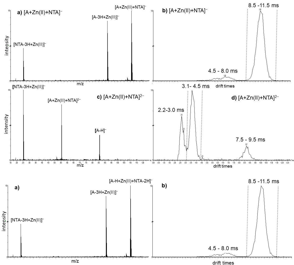
Figure 2. The collision-induced dissociation (CID) of a) [\text{amb}_{5A}\text{-H+Zn(II)+NTA-2H}]^- with 30 V transfer collision energy produced [\text{amb}_{5A}\text{-3H+Ni(II)}]^- and [\text{NTA-3H+Zn(II)}]^- with b) showing the resulting drift time distributions. e) The CID of [\text{amb}_{5A}\text{+Zn(II)+NTA}]^{2-} using 5 V transfer collision energy resulted in the products of [\text{NTA-3H+Zn(II)}]^- and [\text{amb}_{5A}\text{-H}]^- with d) showing the resulting drift time distributions. The dashed lines show the drift time range that were used for determining the relative percent intensity of the precursor and product ions that occurred from the energy-resolved CID inside the transfer collision cell. The other labeled drift times were the products formed at the during the injection of the ternary complex into the entrance beginning of the ion mobility cell.
