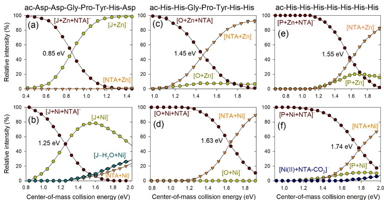
Figure 4. The energy-resolved (c.m./ eV) collision-induced dissociation of [\text{amb}_5\text{-H}+M(\text{II})+\text{NTA-2H}]^- for J , O , and P , where M = \text{Zn} or \text{Ni} , showing the products of [\text{amb}_5\text{-3H}+M(\text{II})]^- , [\text{NTA-3H}+M(\text{II})]^- and [\text{amb}_5\text{-3H-H}_2\text{O}+M(\text{II})]^- . The energy (eV) values shown on the graphs are where there is 50% dissociation of the [\text{amb}_5\text{-H}+M(\text{II})+\text{NTA-2H}]^- complex.
