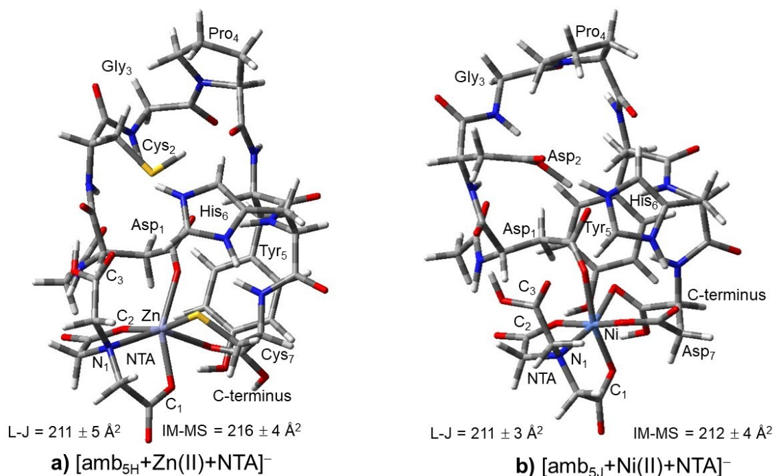
Figure 5. The PM6 geometry-optimized ternary complexes of a) [amb 5H -H+Zn(II)+NTA-2H] - exhibiting Asp 1 - Cys 7 and carboxyl terminus coordination of Zn(II) from amb 5H and amine (N 1 ) and two carboxylates (C 1 and C 2 ) coordination from nitrilotriacetic acid (NTA), b) [amb 5J -H+Ni(II)+NTA-2H] - exhibiting Asp 1 - Asp 7 and carboxyl terminus coordination of Ni(II) from amb 5J and amine (N 1 ) and two carboxylates (C 1 and C 2 ) coordination from NTA. The L-J collision cross sections (CCS He ) for both conformers agree well to their experimentally IM-MS measured CCS He .
