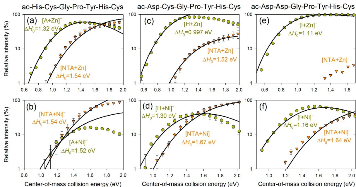
Figure 6. The energy-resolved collision-induced dissociation of [\text{amb}_5\text{-H}+M(\text{II})+\text{NTA}-2\text{H}]^- for A , H , and I , where M = \text{Zn} or \text{Ni} , showing the products of [\text{amb}_5\text{-3H}+M(\text{II})]^- and [\text{NTA}-3\text{H}+M(\text{II})]^- with the CRUNCH threshold fits. The energy (eV) values shown are the dissociation enthalpies ( \Delta H_0 ) at 0 K for the reactions [\text{amb}_5\text{-H}+M(\text{II})+\text{NTA}-2\text{H}]^- \leftrightarrow [\text{amb}_5\text{-3H}+M(\text{II})]^- + \text{NTA} and [\text{amb}_5\text{-H}+M(\text{II})+\text{NTA}-2\text{H}]^- \leftrightarrow [\text{NTA}-3\text{H}+M(\text{II})]^- + \text{amb}_5 .
