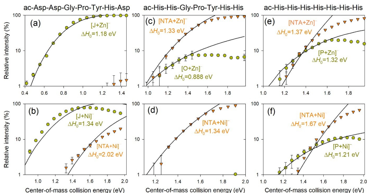
Figure 7. The energy-resolved collision-induced dissociation of [\text{amb}_5\text{-H}+M(\text{II})+\text{NTA-2H}]^- for J , O , and P , where M = \text{Zn} or \text{Ni} , showing the products of [\text{amb}_5\text{-3H}+M(\text{II})]^- and [\text{NTA-3H}+M(\text{II})]^- with the CRUNCH threshold fits. The energy (eV) values shown are the dissociation enthalpies ( \Delta H_0 ) at 0 K for the reactions [\text{amb}_5\text{-H}+M(\text{II})+\text{NTA-2H}]^- \leftrightarrow [\text{amb}_5\text{-3H}+M(\text{II})]^- + \text{NTA} and [\text{amb}_5\text{-H}+M(\text{II})+\text{NTA-2H}]^- \leftrightarrow [\text{NTA-3H}+M(\text{II})]^- + \text{amb}_5 .
