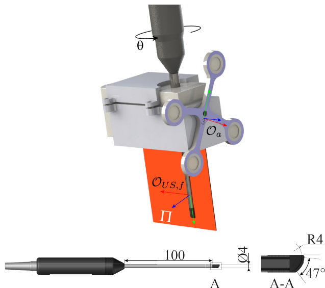
Fig. 1. CAD view of the US probe mounted on a robotic arm and main dimensions of the miniaturized probe. The pose of the robotic arm is tracked by means of a reflective marker.
