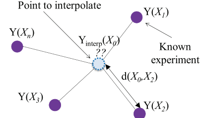
Fig. 6. Kriging interpolation.
