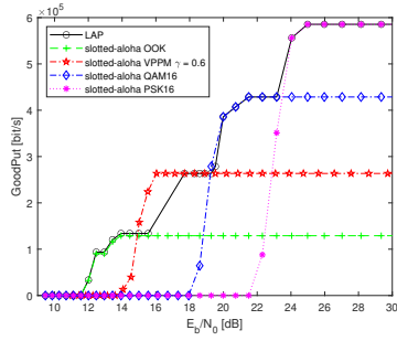
(a) Achieved goodput of LAP and slotted-aloah
