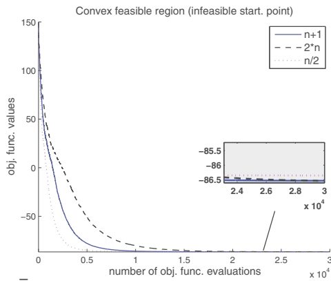
(b) Starting infeasible.
