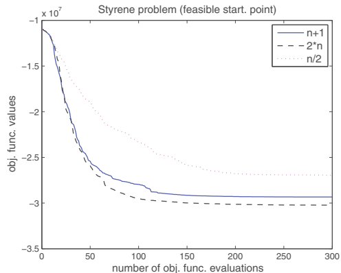
(a) Starting feasible.
