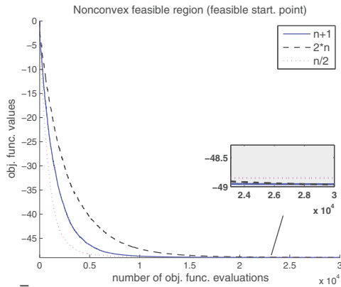
(a) Starting feasible.
