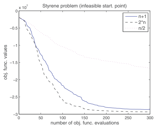
(b) Starting infeasible.
