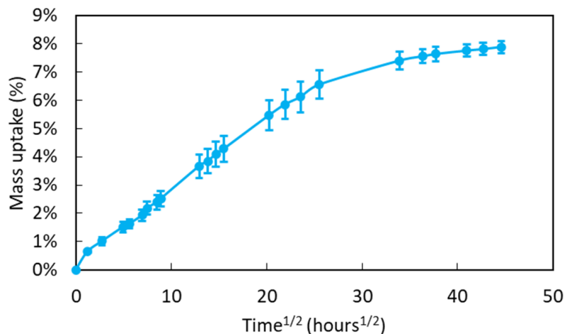
Figure 11. Absorption curve of the bulk adhesive samples immersed in water at 20 °C.
