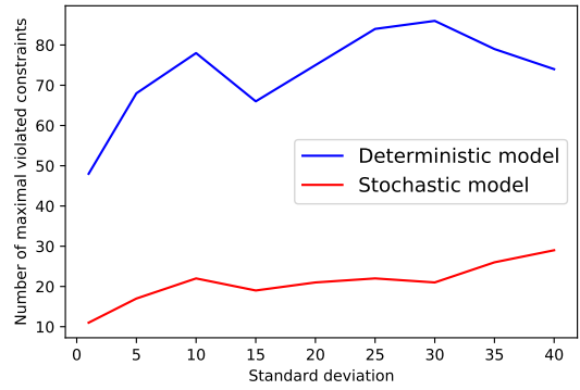
Figure 5: Maximal violated constraints under different standard deviation.
