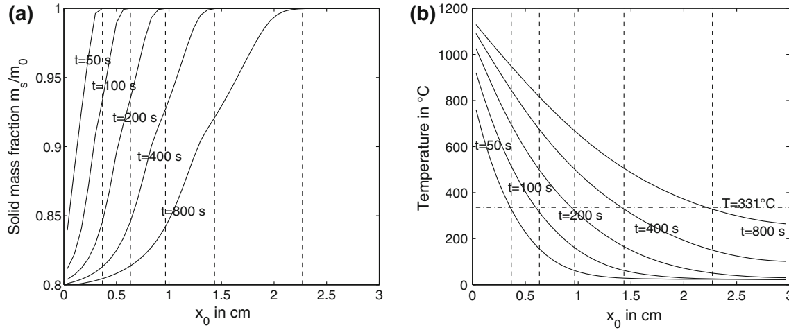
Fig. 4 Comparison of predicted and observed reaction temperature for test case 1. a In plain line the solid mass fraction profile at various times and in dashed line the position where the reaction appears. This position is then reported on b which shows the temperature profile at
