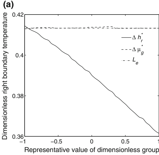
Fig. 7 Evolution of a dimensionless right boundary temperature and b maximum dimensionless pressure with respect to \Delta h_r^* , \Delta \mu_g^* and L_e for thermal decomposition of polymer composite. The value of the
