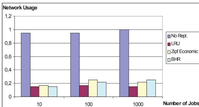
Figure 4 Network usage (see online version for colours)
