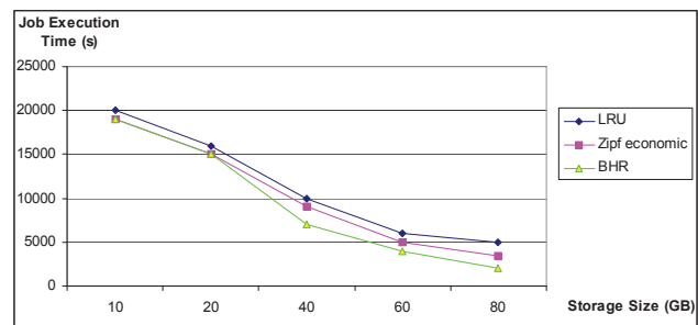
Figure 5 Impact of the storage size on execution times topologies (see online version for colours)
