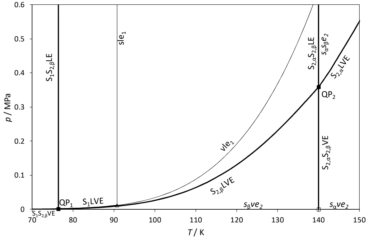
Figure 12. Calculated lowP-lowT global phase diagram of the (1)CH 4 +(2)neo-C 5 H 12 system down to 70 K.
