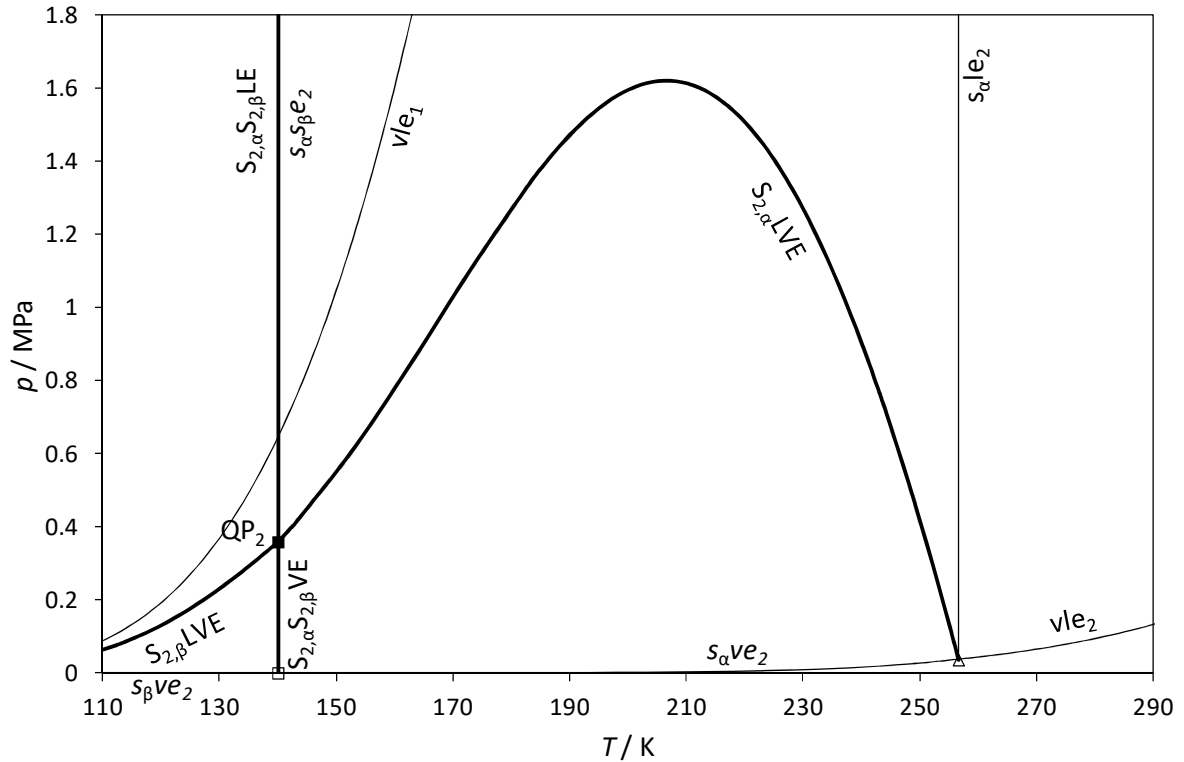
Figure 9. Calculated S_{2\alpha}S_{2\beta}VE , S_{2\alpha}S_{2\beta}LE , S_2LVE , and QP_2 of the (1)CH 4 +(2)neo-C 5 H 12 system.
