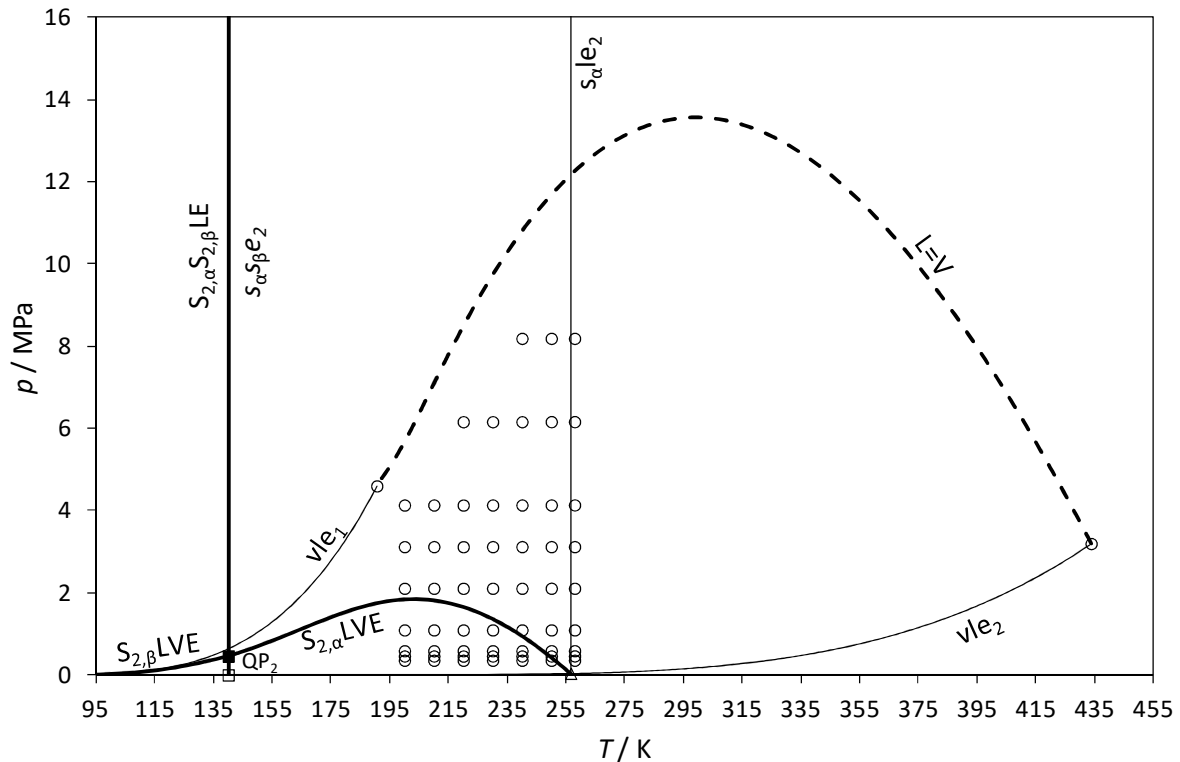
Figure 29. Calculated global phase diagram of the (1)CH 4 +(2)neo-C 5 H 12 system down to 95 K.
