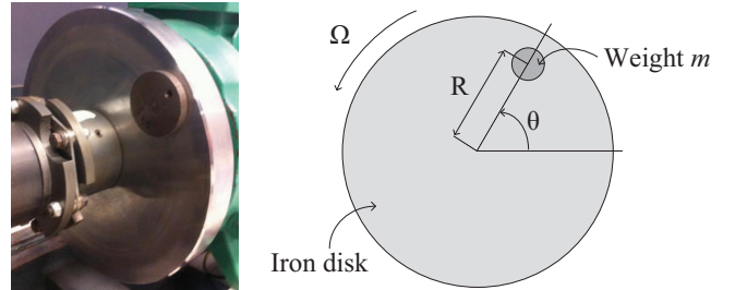
Fig. 7. Photography (left) and schematic representation (right) of the iron disk used to generate the three levels of mechanical unbalance B_1 , B_2 and B_3 . The different weights m_1 , m_2 and m_3 are attached on the iron disk at a distance R from the rotation axis in order to generate the desired level of mechanical unbalance.
