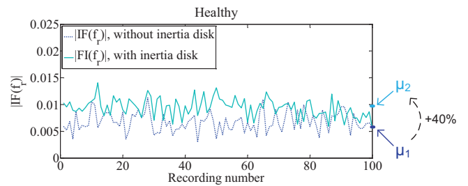
Fig. 9. Fault signature |IF(f_r)| during healthy conditions with different configuration of the monitored system : with the inertia disk (light blue solid line) and without the inertia disk (dark blue dotted line).
