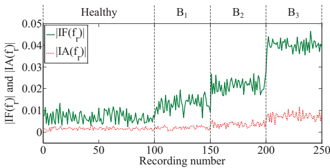
Fig. 8. Illustration of |IF(f_r)| (green solid line) and |IA(f_r)| (red dotted line) evolutions for the different health states of the induction machine (healthy, B_1 , B_2 and B_3 ).
