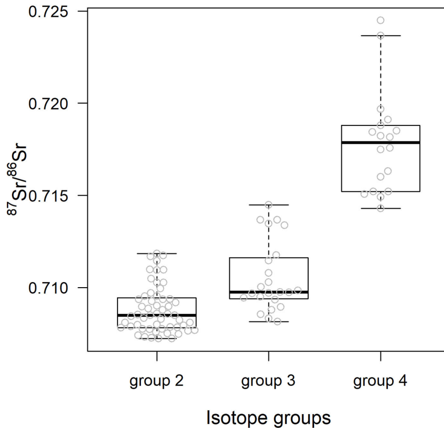
FIGURE 5 | ^{87}\text{Sr}/^{86}\text{Sr} values of the biological samples according to the isotope group of the lithological unit underlying the sample sites. Center line and box edges are, respectively the median and the 1st and 3rd quartiles, and whiskers represent data points within the range quartile \pm 1.5 (interquartile range). Raw values are displayed with gray dots.
