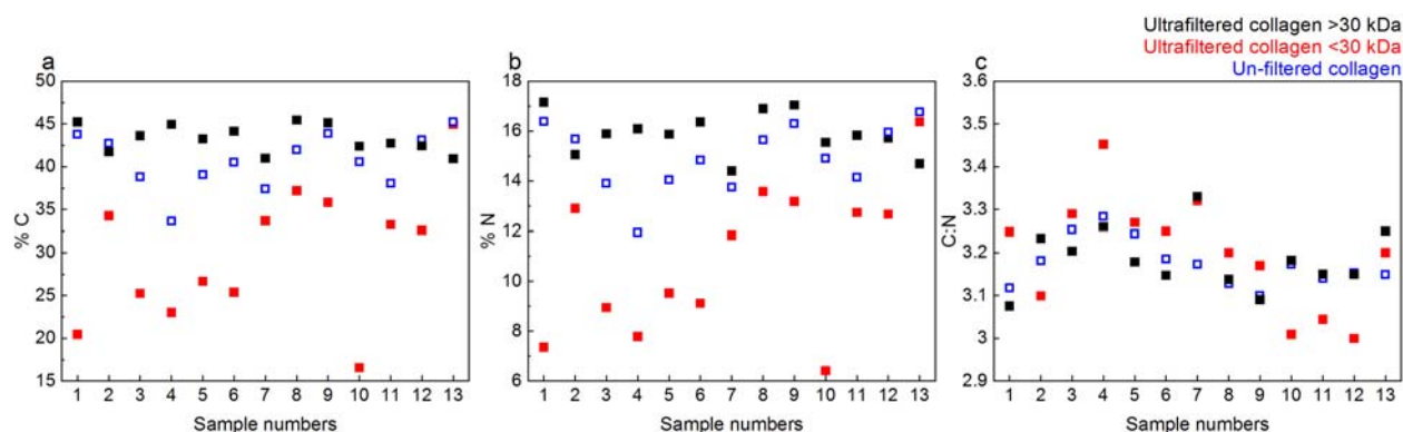
Figure 10. %C, %N, and C:N ratios of collagen extracts in Experiment B: >30 kDa fraction (black), <30 kDa fraction (red) and Method 3 extracts without ultrafiltration (blue). Instrumental error is ±0.2%.
