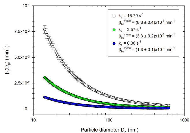
Figure 3. Distribution of the wall loss coefficient \beta_i ( D_p ) for three values of k_e obtained experimentally: 16.70 \text{ s}^{-1} (white), 2.57 \text{ s}^{-1} (green) and 0.36 \text{ s}^{-1} (blue).
