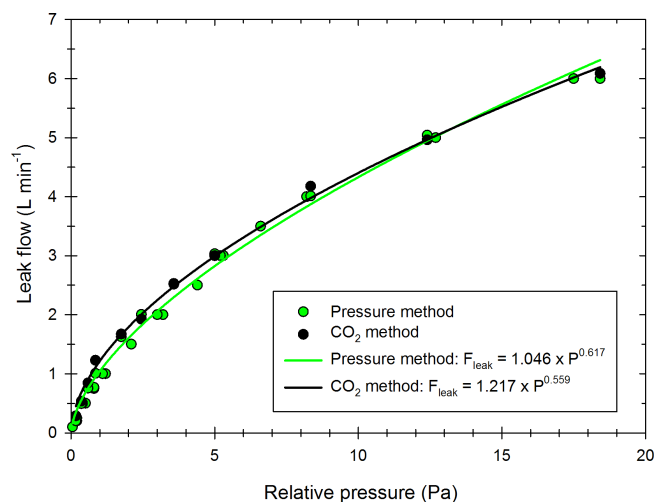
Figure 2. Values of the leak flow as a function of relative pressure, obtained with the “pressure method” (green) or the “CO 2 method” (black). The dots represent the experimental results, and the curves represent the mathematical simulation for both methods.
