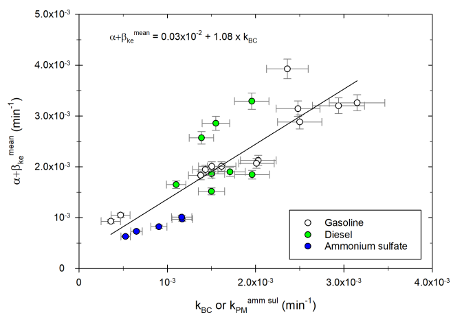
Figure 5. Mean loss coefficient \alpha + \beta_{k_c}^{\text{mean}} as a function of the decay coefficient k_{\text{BC}} or k_{\text{PM}}^{\text{amm sul}} obtained for the “neutralized wall” chamber experiments performed with particles from diesel (green) and gasoline (white) engines or ammonium sulfate particles (blue). A linear fit of the data is shown (black line).
