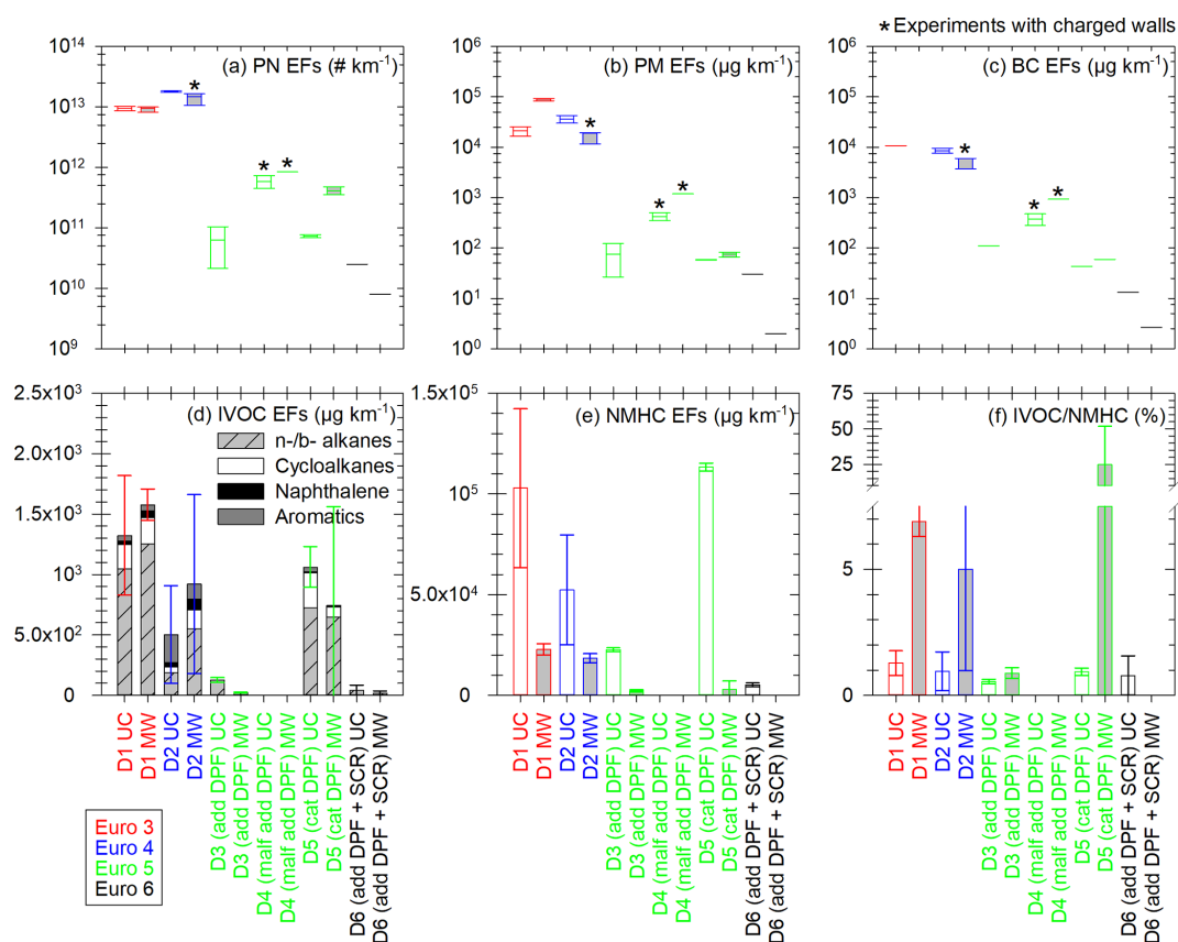
Figure 6. Emission factors of PN (a), PM (b), BC (c), IVOCs (d) and NMHCs (e), and IVOC / NMHC ratio (f) for the six tested Euro 3–6 diesel vehicles UC (white) and MW (light grey) conditions. IVOC EFs (d) are the sum of EFs of linear and branched (n- and b-, respectively) alkanes (hatched grey), cycloalkanes (white), naphthalene (black) and aromatics (dark grey), with retention times in the range corresponding to C 12 –C 22 alkanes. EFs are given in \mu\text{g km}^{-3} and the IVOC / NMHC ratio in percentage. Vehicles are sorted by Euro norm: Euro 3 in red, Euro 4 in blue, Euro 5 with add or cat DPF in green and Euro 6 in black. The Euro 5 vehicle showing signs of malfunctioning DPF is referred to as “D4 (malif add DPF)”. The boxes represent the 25th and 75th percentiles. The solid line in panels (d) to (f) represents the median. The whiskers are the 10th and 90th percentiles. Error bars represent 1 standard variation in panels (d) to (f). Panel (f) has a broken axis to better show the smaller values. The boxplots with the sign * represent the cycles for which chamber initial concentrations can be impacted by electrostatic charge on the walls. It could only impact PN, PM and BC, since IVOCs and NMHCs were sampled directly from emissions.
