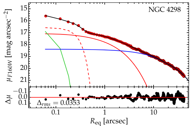
Figure 9. Similar to Figure 1, but for NGC 4298.
