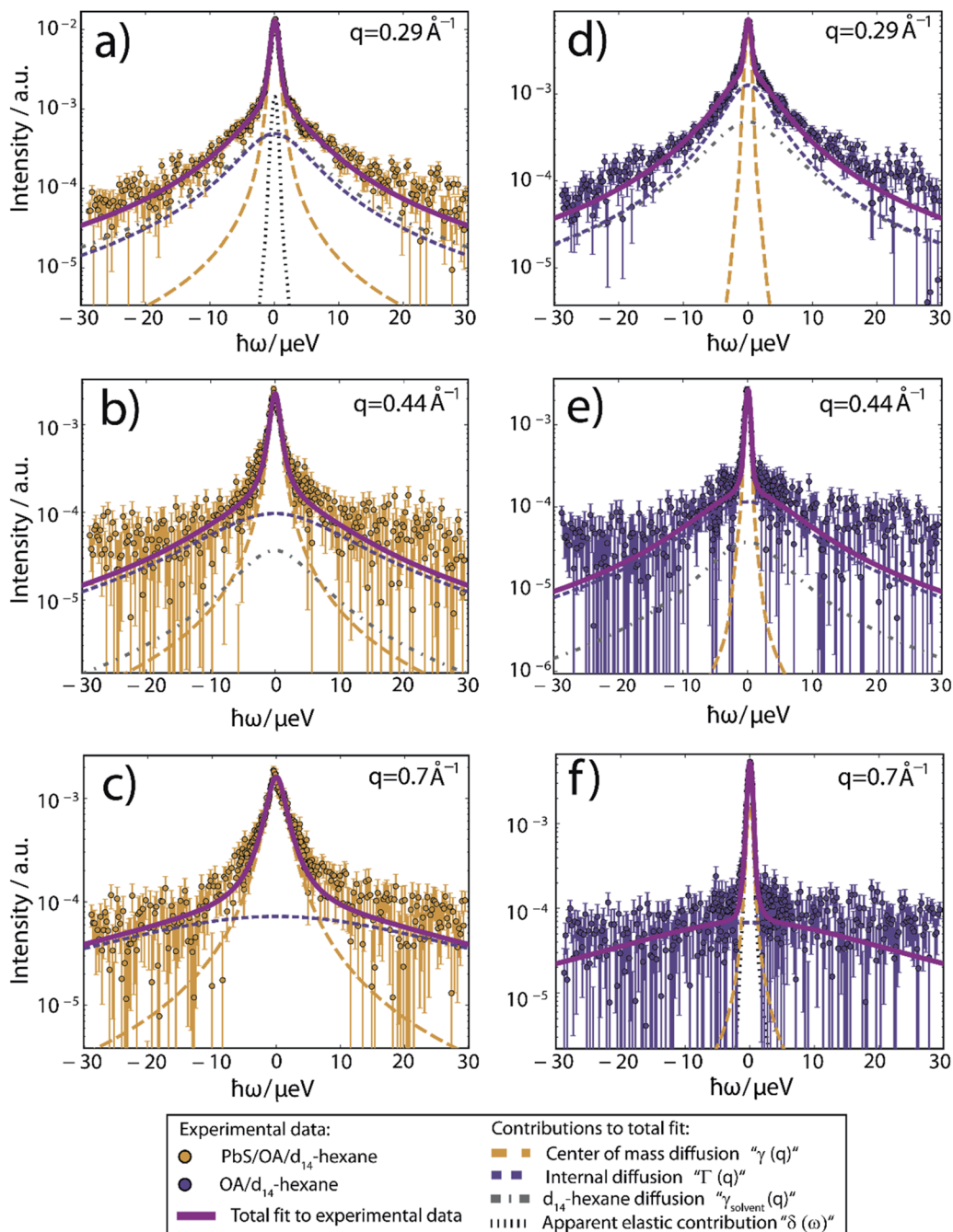
Fig. 2 QENS spectra at T = 239 K and three different scattering vectors. (a–c) Experimental data of PbS/OA/ d_{14} -hexane and (d–f) of OA/ d_{14} -hexane. A sloped background arising from instrument and sample contributions has been subtracted in all cases. Solid lines represent fits to the experimental data, composed of the Lorentzian contributions from the center-of-mass diffusion, internal diffusion, d_{14} -hexane solvent and an apparent elastic contribution represented by dashed lines according to the model described by eqn (1) in the ESI.† The apparent elastic contribution and the d_{14} -hexane diffusion are not visible on all plots due to the low signal and rapid broadening of the d_{14} -hexane signal with rising q . The d_{14} -hexane contribution has been rescaled by the effective excluded volume of OA. All data has been binned by pairs of two channels for small ( |\hbar\omega| < 5.85 \mu\text{eV} ) and by groups of four channels for large absolute values of the energy transfer, respectively, subsequent to fitting for better visibility.
