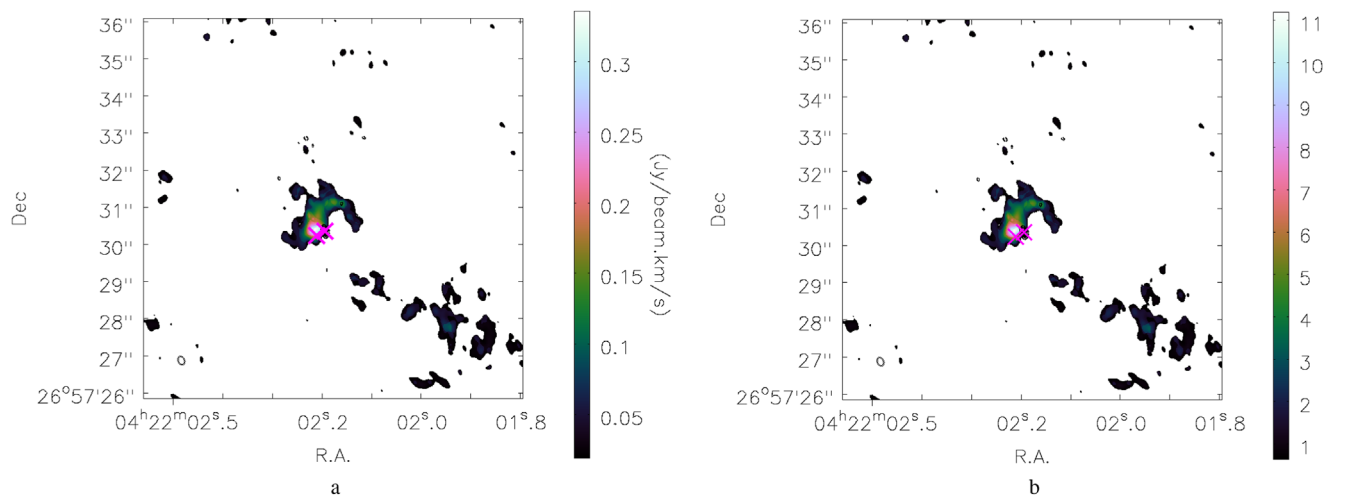
Figure 7. (a) ALMA CO 2–1 redshifted component moment 0 images, corresponding to velocities of 8.17–16.43 \text{km s}^{-1} , with a large ( 10'' \times 10'' ) FoV. (b) S/N map of (a).
