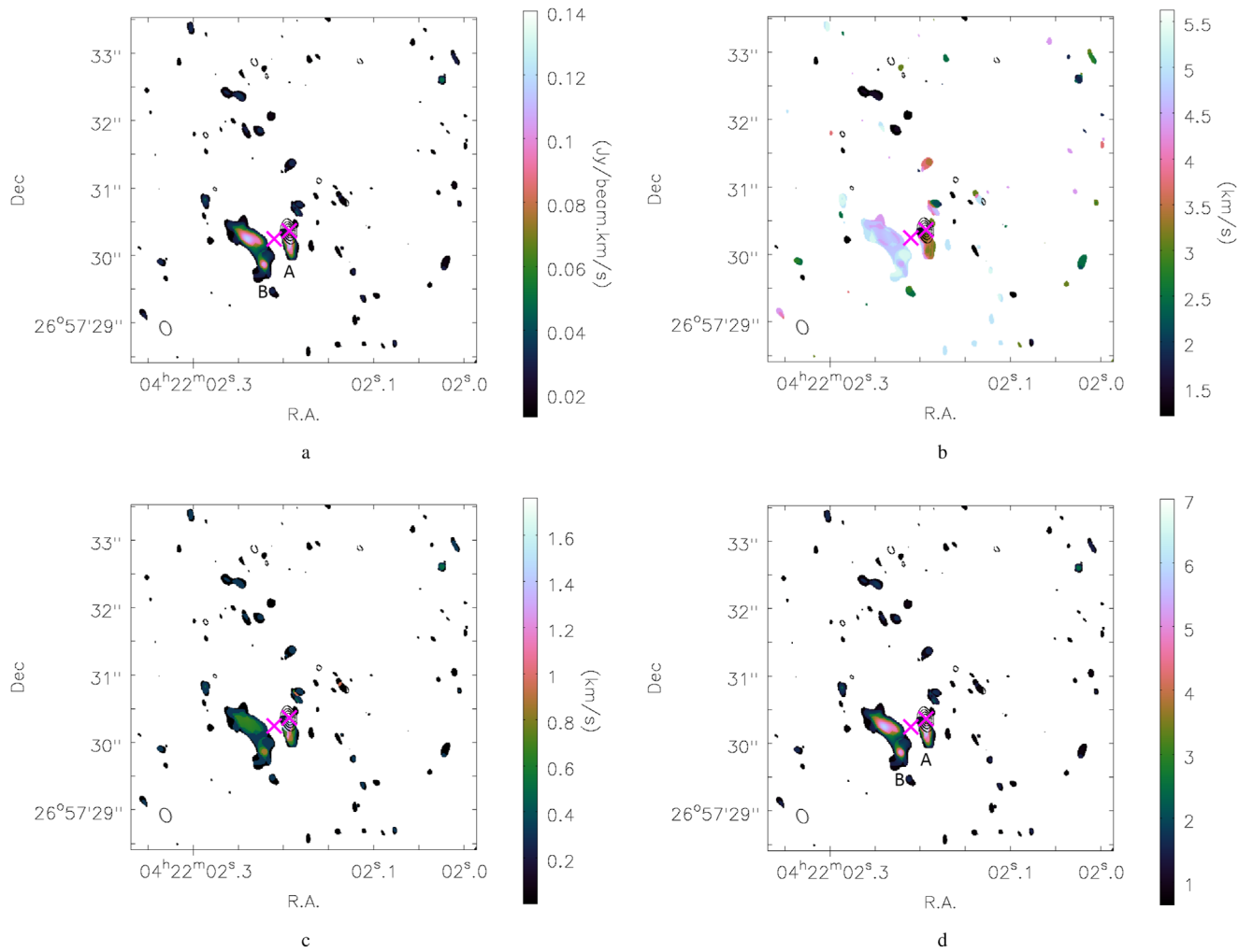
Figure 6. ALMA CO 2–1 blueshifted component images, corresponding to velocities of 1.19–5.64 \text{km s}^{-1} . (a) ALMA CO 2–1 moment 0 image of the FS Tau A blueshifted component. (b) ALMA moment 1 image of the FS Tau A blueshifted component. (c) ALMA moment 2 image of FS Tau A blueshifted component. (d) S/N map of (a). The black contours in the images represent the continuum emission image showing the position of the central stars, showing 0.2, 0.4, 0.6, and 0.8 of the peak intensity 2.08 \text{ mJy beam}^{-1} . The red crosses show the positions of FS Tau Aa and Ab derived from our near-infrared observations, respectively, assuming that the peak of the continuum emission corresponds to Aa.
