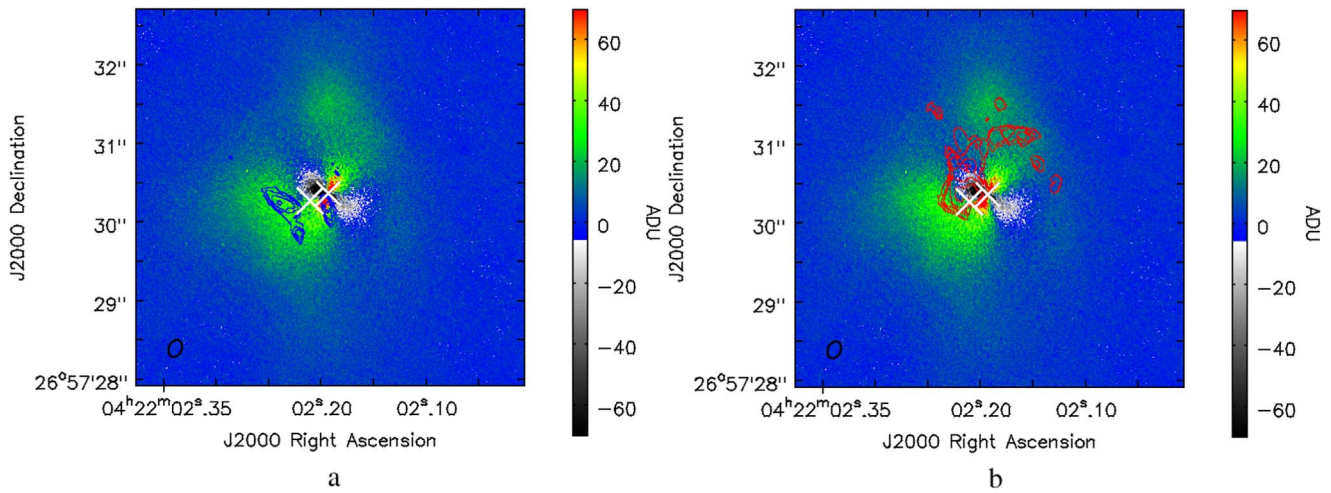
Figure 9. (a): Q_\phi image (color scale) with the ALMA CO 2–1 blueshifted component image (contour) overlotted. Contours are 0.03822, 0.06374, 0.08926, and 0.1148 Jy beam -1 ; (b): Q_\phi image (color scale) with the ALMA CO 2–1 redshifted component image (contour) overlotted. Contours are 0.0606, 0.0883, 0.116, 0.144, and 0.227 Jy beam -1 .
