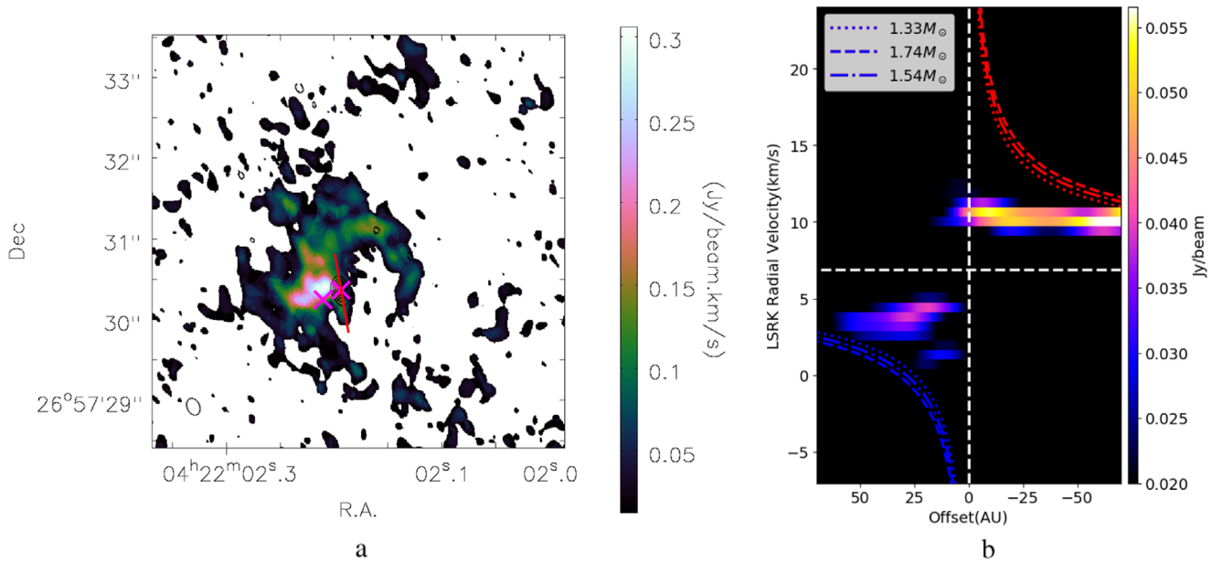
Figure 10. (a) ALMA CO 2–1 moment 0 image of FS Tau A, including both the blueshifted and redshifted components. The red line shows the radius and position angle of the generated P–V map. (b) P–V map of the FS Tau A ALMA CO 2–1 image central region. The image is drawn along a slit with a position angle of 9^{\circ}9 , a radius of 0''.5 (70 au), and a width of 1 pixel. The blue and red lines show the blueshifted and redshifted Keplerian rotation curves, respectively, assuming an LSRK radial velocity of 6.9 \text{ km s}^{-1} . The horizontal dashed line shows an LSRK radial velocity of 6.9 \text{ km s}^{-1} and the vertical line corresponds to an offset of 0 au.
