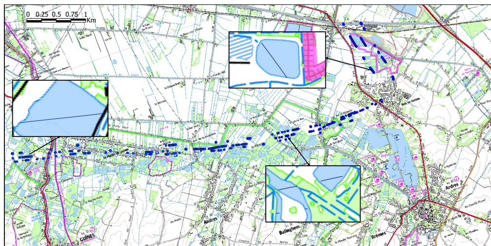
Figure 15. The detected water body surfaces using our proposed radar technique for the area between Guïnes and Ardres. The specular points of reflection, represented by a blue coloring, are superimposed on IGN maps.
