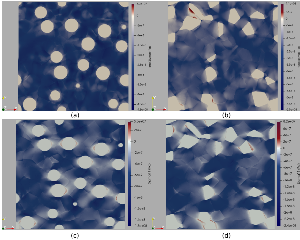
Figure 9: Stress fields at the end of the simulation for f_p = 15\% . d_p \approx d_g , T = 1400^\circ\text{C} , and |\dot{E}| = 10^{-7} \text{ s}^{-1} . Hydrostatic compression, maps of tr(\boldsymbol{\sigma}) (a) for a Voronoi-type microstructure with spherical, (b) for a Laguerre-type microstructure with polyhedral voids. Uniaxial compression, maps of \sigma_{11} (c) for a Voronoi-type microstructure with spherical voids, (d) for a Laguerre-type microstructure with polyhedral.
