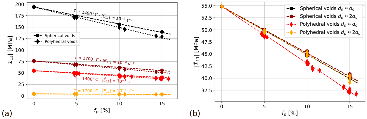
Figure 5: Stress versus porosity for Voronoi-type microstructures with spherical voids, Laguerre-type and Voronoi-type microstructures with polyhedral voids, submitted to a uniaxial compression loading (dotted and dashed lines are linear regression functions). (a) d_p \approx d_g for different temperatures and strain rates, (b) d_p \approx d_g and d_p \approx 2d_g for T = 1400^\circ\text{C} and |\dot{\epsilon}_{11}| = 10^{-7} \text{ s}^{-1} .
