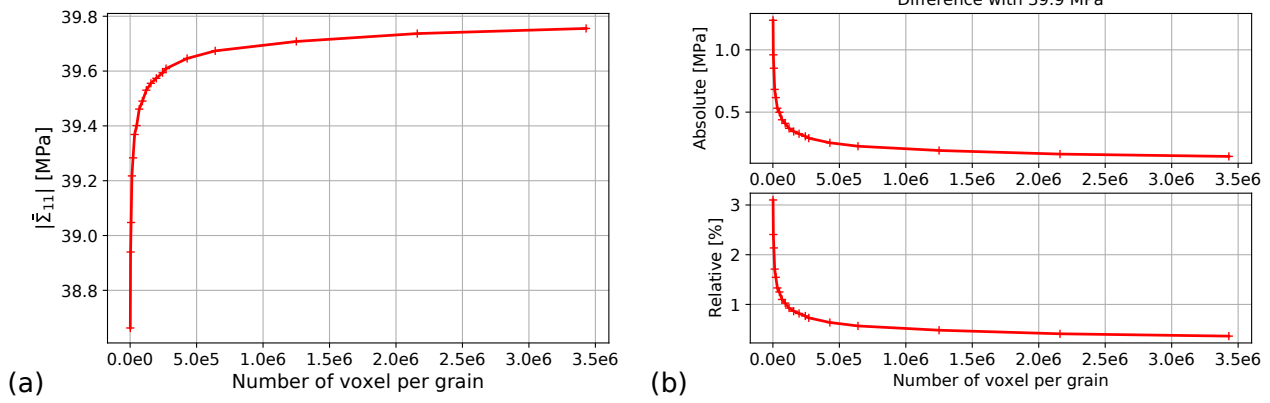
Figure A.1: (a) Effective stress on a 100 grains Voronoi-type microstructure with 15 polyhedral voids, at 1900°C and 10^{-3} \text{ s}^{-1} , under uniaxial compression. (b) Absolute and relative differences of each simulation results with 39.9 MPa.
