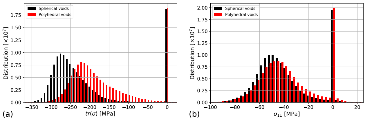
Figure 10: Distribution of stress at the end of the simulation for f_p = 15\% in Voronoi-type microstructure with spherical voids and Laguerre-type microstructure with polyhedral voids. d_p \approx d_g , T = 1400^\circ\text{C} , and |\dot{E}| = 10^{-7} \text{ s}^{-1} . (a) tr(\boldsymbol{\sigma}) for hydrostatic compression loading, (b) \sigma_{11} for uniaxial compression loading.
