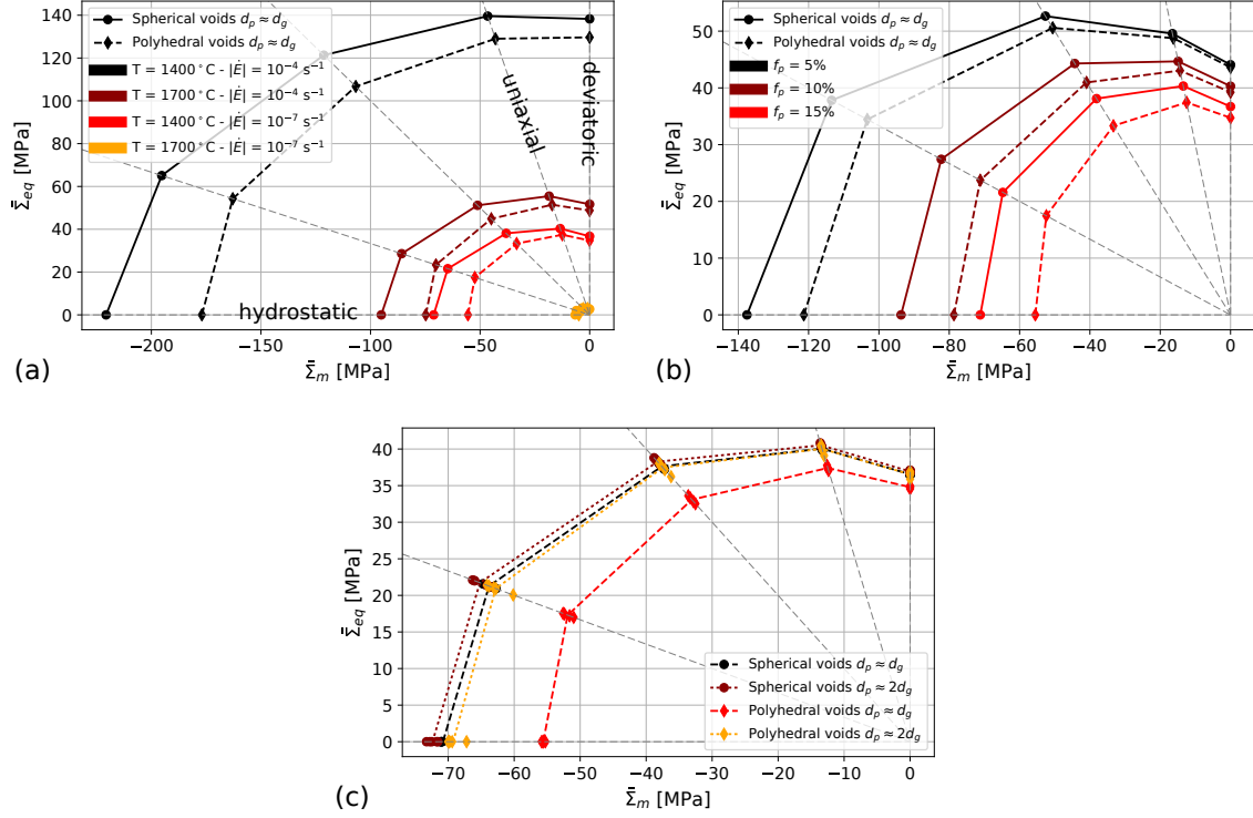
Figure 6: Equivalent stress versus hydrostatic stress of Voronoi-type microstructures with spherical voids, Laguerre-type microstructures with polyhedral voids (dotted and dashed lines are interpolations between the mean values obtained for each stress triaxiality) (a) for different temperatures and strain rates with d_p \approx d_g and f_p = 15\% , (b) for different porosities with d_p \approx d_g , T = 1400^\circ\text{C} , and |\dot{E}| = 10^{-7} \text{ s}^{-1} , (c) for d_p \approx d_g and d_p \approx 2d_g with f_p = 15\% , T = 1400^\circ\text{C} , and |\dot{E}| = 10^{-7} \text{ s}^{-1} .
