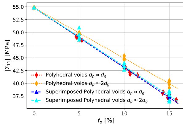
Figure 8: Stress versus porosity for T = 1400^\circ\text{C} and |\dot{E}_{11}| = 10^{-7} \text{ s}^{-1} . Voronoi-type and Laguerre-type microstructures with polyhedral voids (red). Laguerre-type microstructures with polyhedral voids (orange). Laguerre-Voronoi-type microstructures with polyhedral voids (dark blue and light blue). Dotted and dashed lines are linear fit functions.
