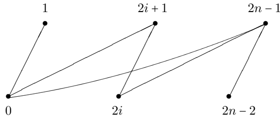
Figure 2: The Hasse diagram of Q_{2n} .
