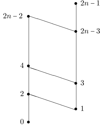
Figure 3: The Hasse diagram of R_{2n} .
