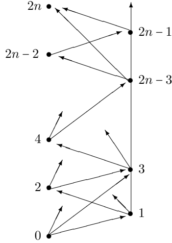
Figure 1: The digraph H_{2n+1} .
