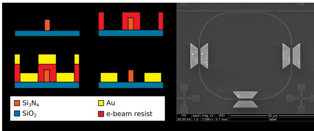
Figure 4.a image of the process to build a HPWG, lift-off. 4.b scanning electron microscopy image of the manufactured ring resonator
