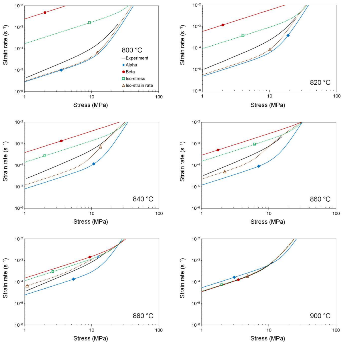
Figure 11: Strain rate as a function of stress, from 800 to 900 °C, experimental results on M5 Framatome flat specimens, predictions from single- \alpha and single- \beta creep laws and from iso-stress and iso-strain rate homogenisation models.
