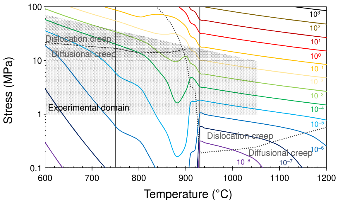
Figure 13: High Stress-temperature map with strain rate isovalue curves (in s^{-1} ) for M5 Framatome alloy – Model predictions, from axial tensile creep tests on sheet specimens (grey region: experimentally investigated domain). Dashed and dotted lines respectively delineate the competition between dislocation creep and diffusional creep regimes for the \alpha and \beta phases, respectively. Continuous vertical lines delineate boundaries between near- \alpha and (\alpha + \beta) , and (\alpha + \beta) and full \beta domains, respectively.
