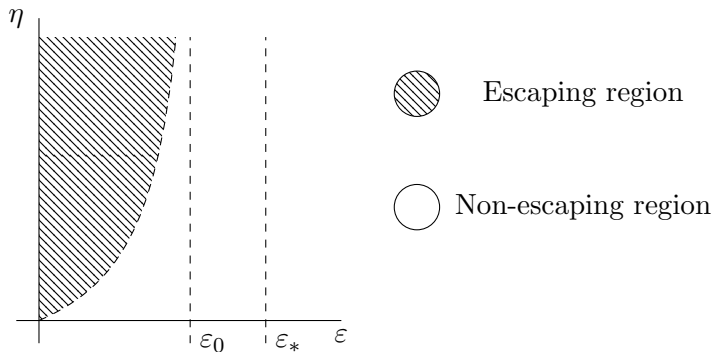
FIGURE 1. Radial critical points of the extended functional E_{\varepsilon,\eta} when W'(1) > 0 and \tilde{W}'(0) > 0 . In the escaping region, there is a co-existence of non-escaping and escaping critical points. In the non-escaping region, only the non-escaping critical point exists.
