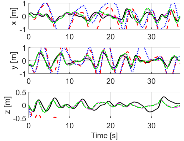
Figure 6: Validation flight dataset: Position \xi^I of the UAV along x^I , y^I and z^I . Measurements are in thick black line, output of model \mathcal{M}_0 in red dashed line, \mathcal{M}_1 in blue dotted line, \mathcal{M}_2 in thin magenta line, \mathcal{M}_{lin} in green dotted-dashed line.
