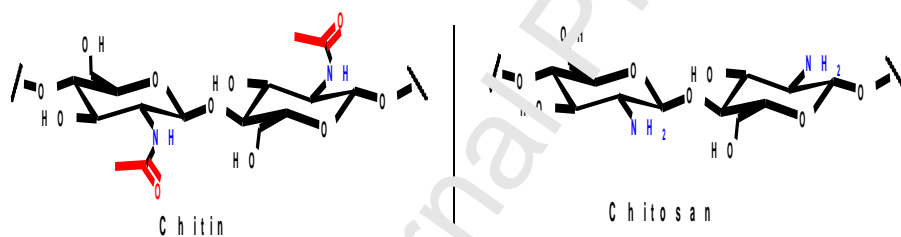
Figure 2. Theoretical chemical structures of chitin and chitosan.
