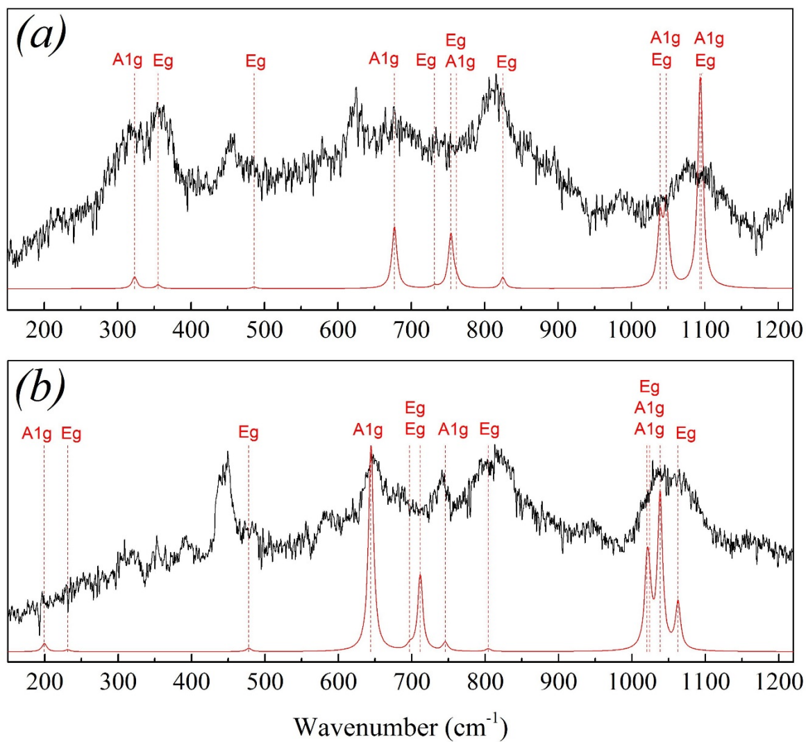
Figure 3 Experimentally observed (solid lines) and LCAO calculated (red lines) Raman bands of \text{B}_{12}\text{S} (a) and \text{B}_{12}\text{Se} (b) at ambient conditions. The positions of the predicted Raman peaks are traced by red dashed lines, the corresponding phonon modes are indicated.
