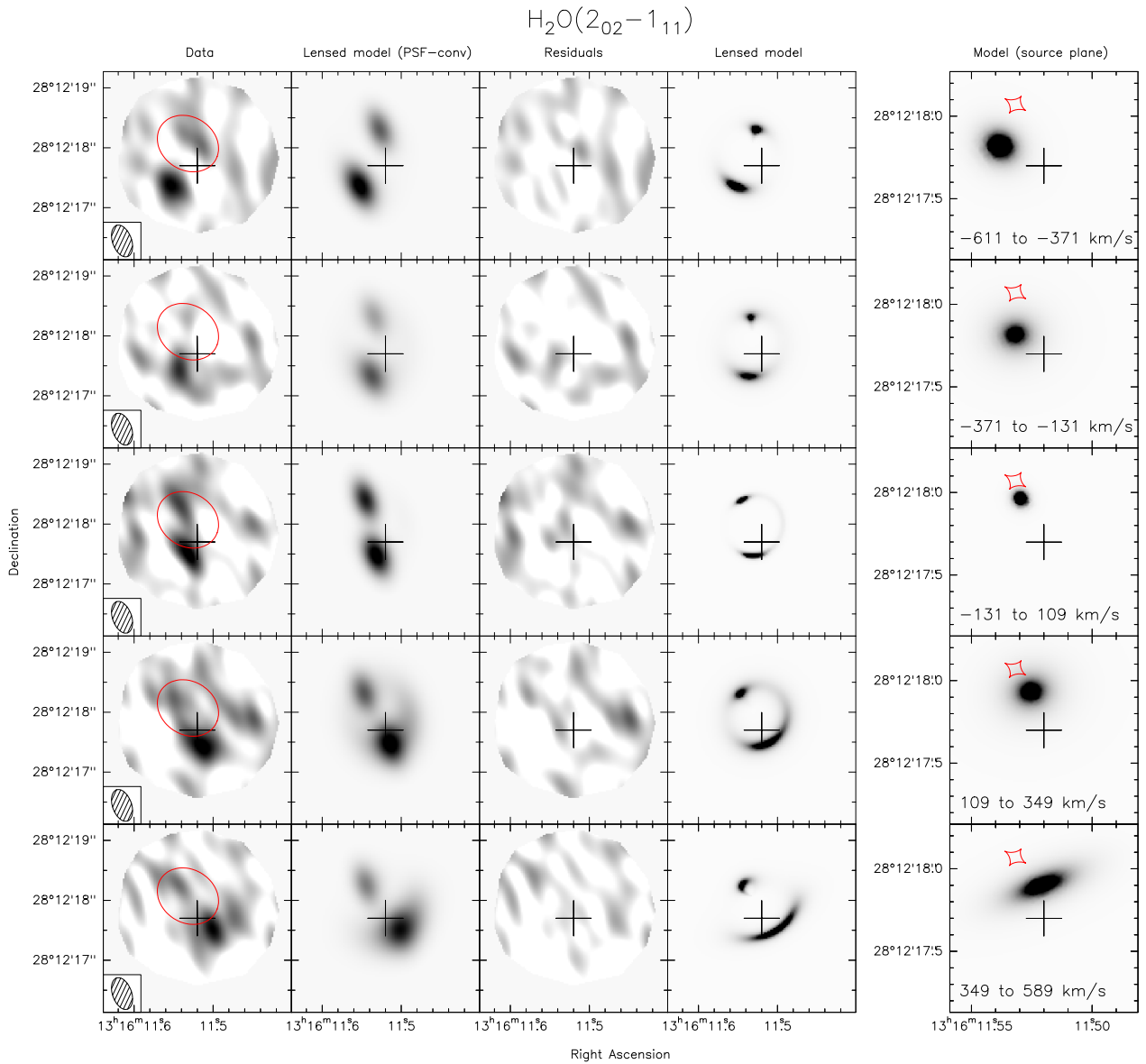
Fig. A.4. Lens modeling of the \text{H}_2\text{O}(2_{02}-1_{11}) spectral channels. The velocity ranges covered by each channel are marked in the right-hand panels . See Fig. A.3 for further details.
