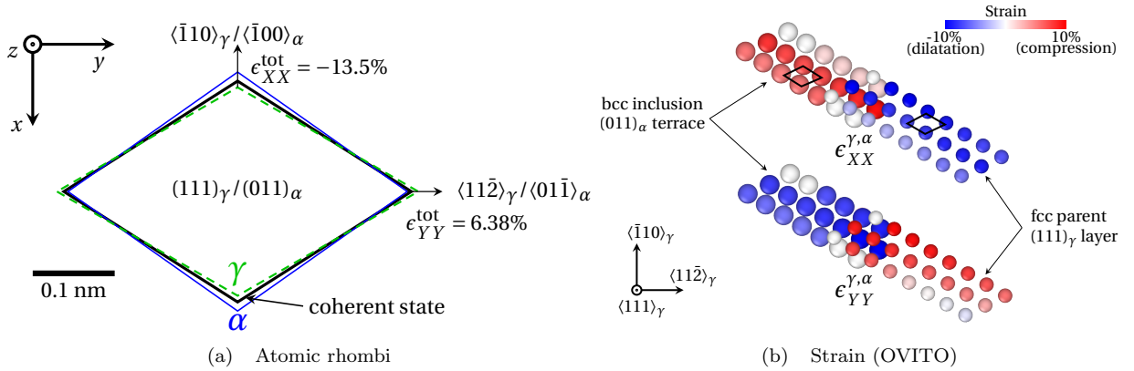
Figure 8: Misfit strain at the coherent (011)_\alpha \parallel (111)_\gamma inclusion terrace expressed in the terrace plane coordinate frame ( \langle \bar{1}10 \rangle_\gamma, \langle 11\bar{2} \rangle_\gamma, \langle 111 \rangle_\gamma ). (a) Scale drawing of the atomic rhombi in the terrace plane. Blue lines represent the unstrained bcc structure, green dashed lines the unstrained parent crystal, and bold black lines the coherent state. (b) QA calculation ( t = 1500 ) at one (011)_\alpha coherent terrace. Top: \epsilon_{XX}^{\gamma,\alpha} . Bottom: \epsilon_{YY}^{\gamma,\alpha} . In (b) the strain was calculated using OVITO (finite strain theory).
