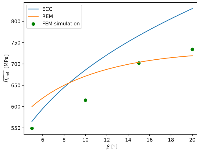
Figure 8 Hardness for all models and various contact angles for a material with E = 210 GPa, \sigma_Y = 102 MPa and n = 0.2 .
