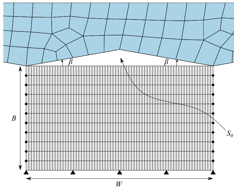
Figure 4 Schematic of the multiple wedges indentation geometry. The indenter is shown in blue and the substrate in grey. The mesh represented here is coarser than that used in the simulations for clarity.
