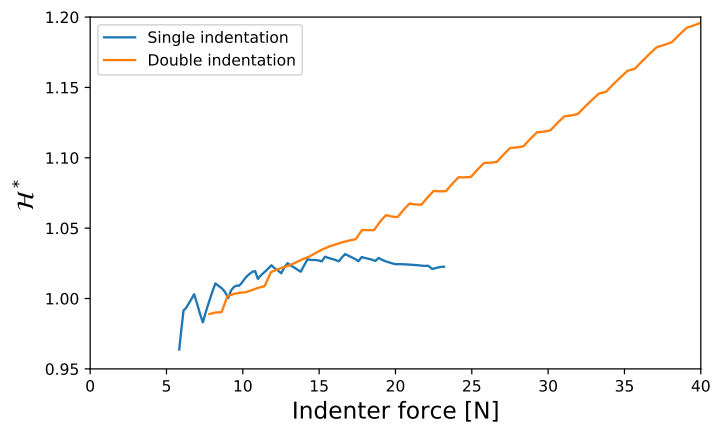
Figure 9: Comparison of the computed instantaneous hardness between single and multiple wedges indentation.
