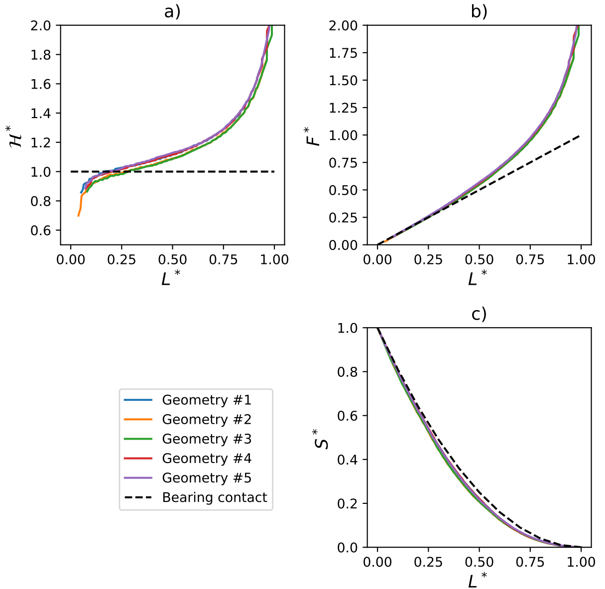
Figure 12: Influence of the geometrical parameters (see Tab. 1) on multiple wedges indentation. The results from the bearing contact model are given as dashed lines.
